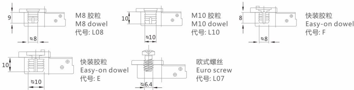
φ35mm铰杯可配螺丝种类 (Options of screws and dowels)
