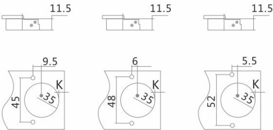
φ35mm铰杯种类 (Hing cup types)
