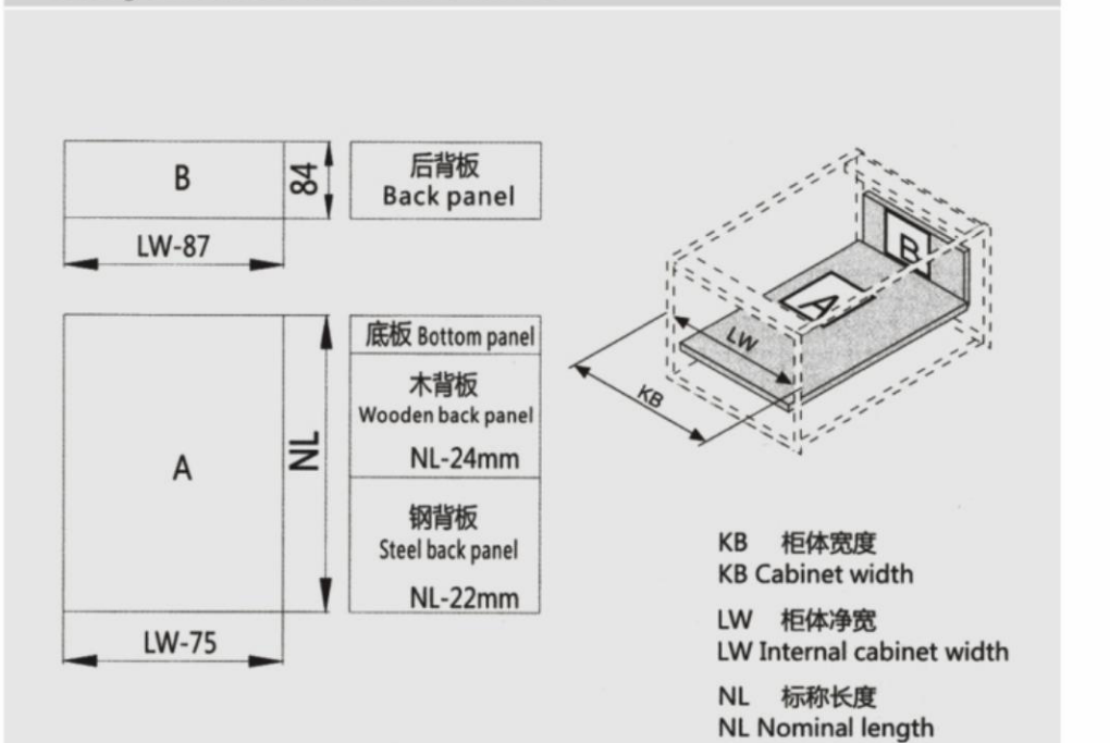
16mm 厚的密度板裁切尺寸 Cutting dimensions for 16mm-thick MDF
