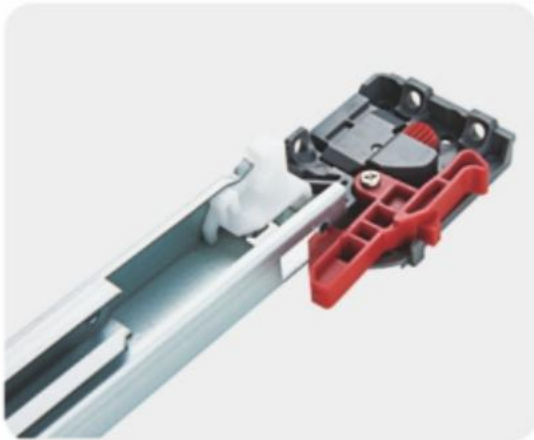
三维可调连接件 3D adjustment connector
